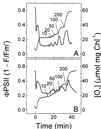
Fig. 2. Simultaneous measurements of PSII efficiency (estimated as 1 - F/F_m' , solid line) and \text{O}_2 evolution (dotted line) in dark-adapted cells of C. reinhardtii (CW92, A) and the Cia3 /CW15 mutant (B). Cells resuspended with \text{CO}_2 -free 20 mM MES-KOH (pH 5.3) were dark-adapted for 5 min and then subjected to continuous illumination by light saturating for photosynthesis ( 750 \mu\text{mol photons}/\text{m}^2/\text{s} ). When cells showed no net \text{O}_2 evolution, various concentration of \text{HCO}_3^- were added where indicated by arrows labeled with numbers in \mu\text{M} .
